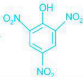
2,4,6-Trinitrophenol (Picric acid)
